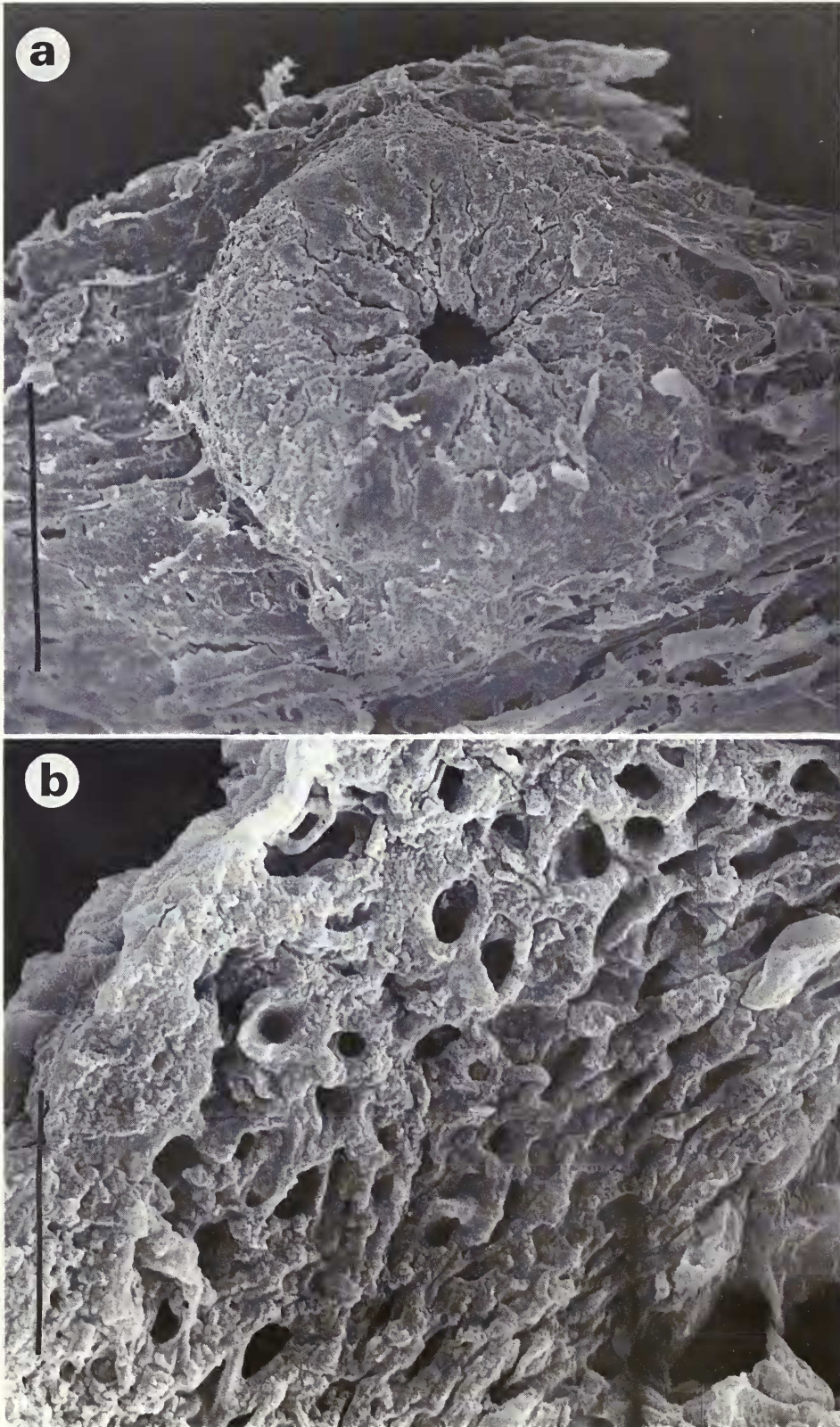
Fig. 71 Odontura raphidospora (Rehm) Clem. (S-lectotype of Leptorhaphis pyrenopezizoides ) (a) Surface view of ascoma; scale = 176 \mu\text{m} ; (b) Detail of exciple: pseudoparenchymatous tissue of leptodermatous cells in places, not neat textura angularis ; scale = 8.6 \mu\text{m} .
